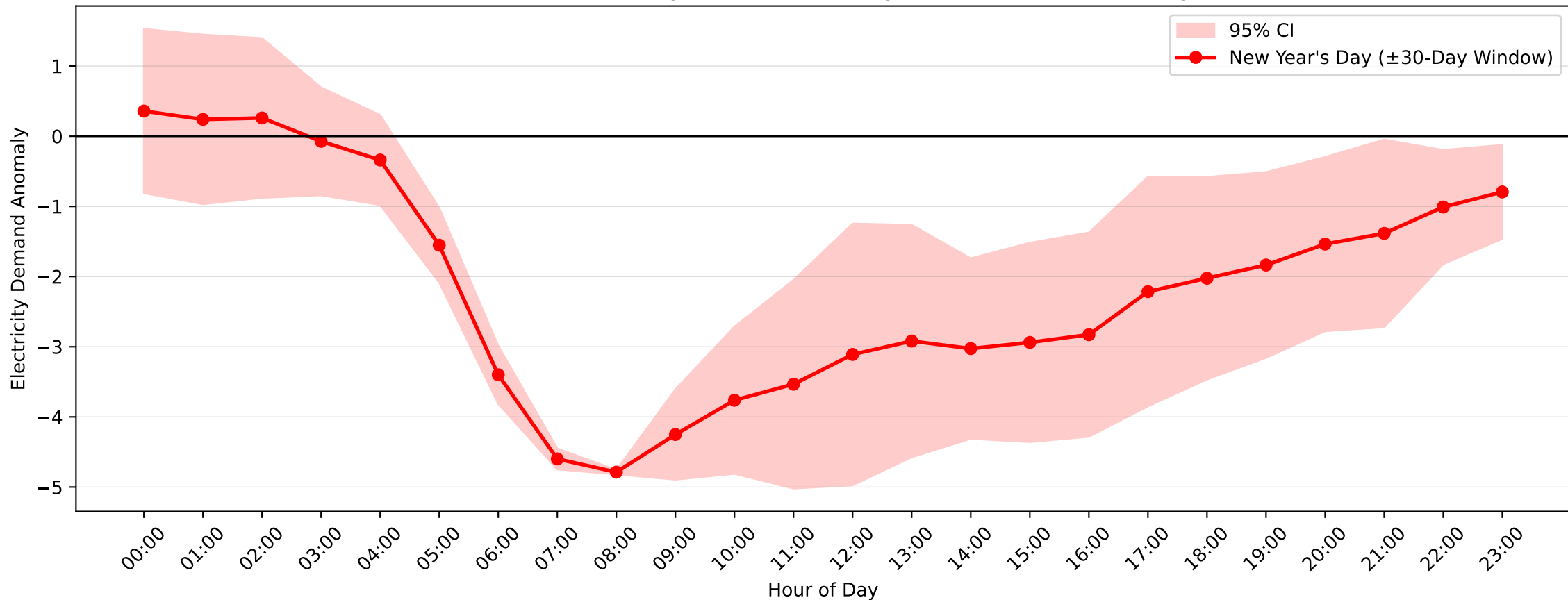
Kirrawee Demand Anomaly: New Year's Day (2013-2014, \pm 30 -Day Window)
