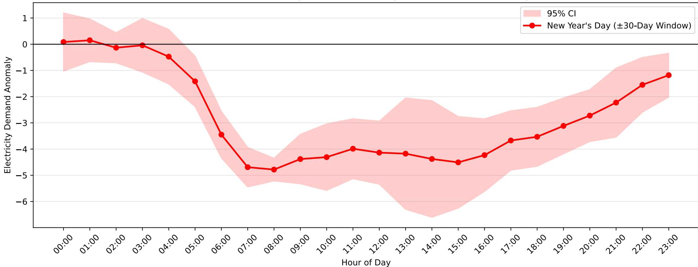
Kirrawee Demand Anomaly: New Year's Day (2016-2017, \pm 30 -Day Window)
