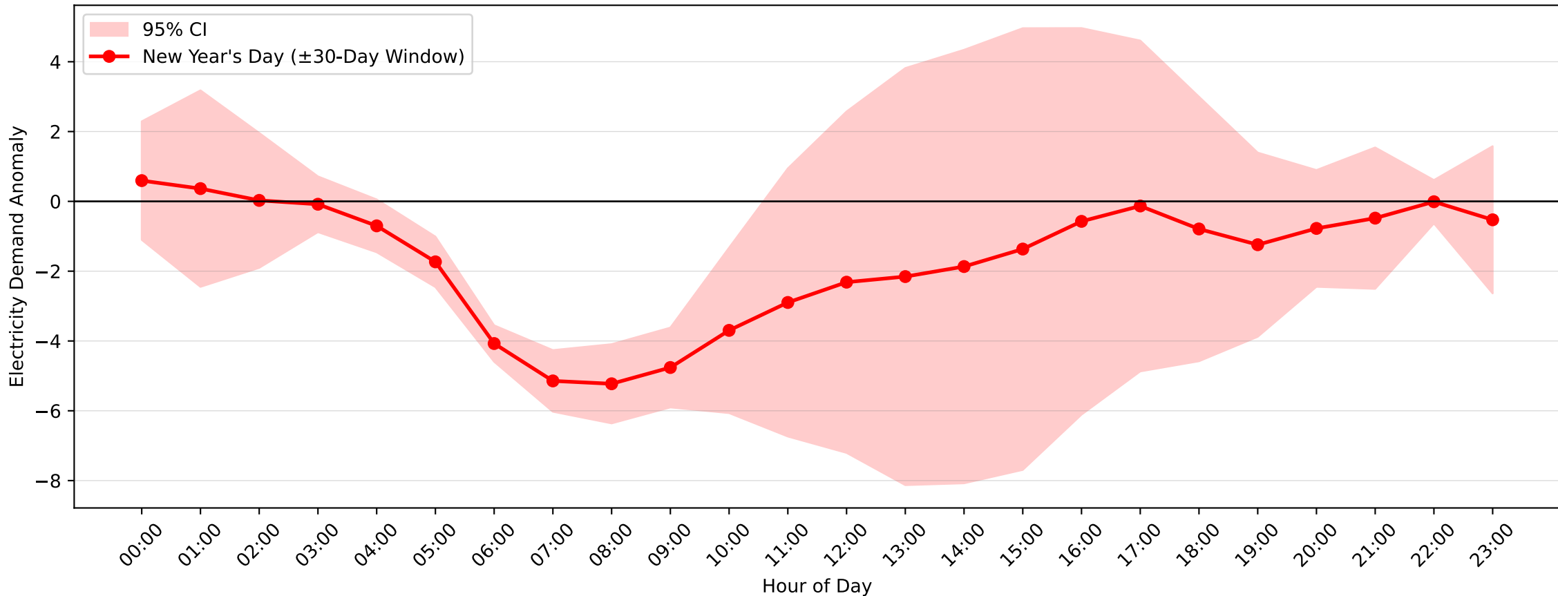
Kirrawee Demand Anomaly: New Year's Day (2010-2011, \pm 30 -Day Window)
