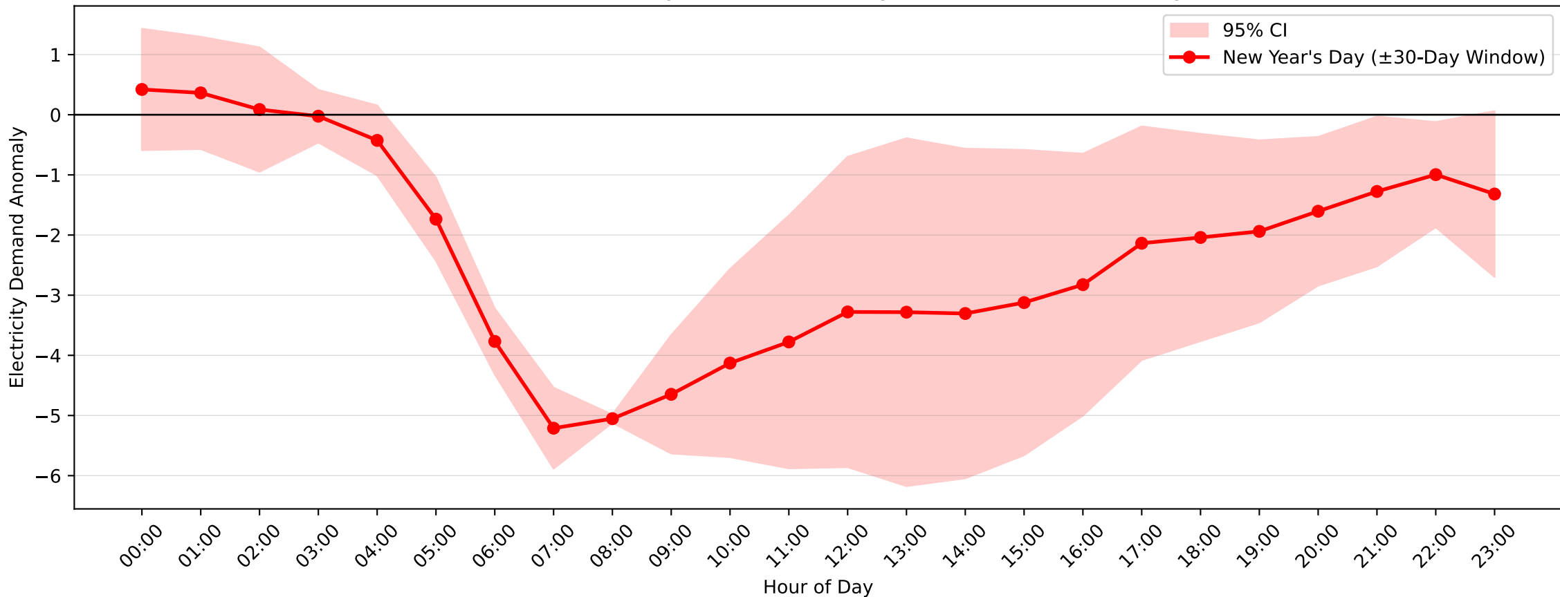
Kirrawee Demand Anomaly: New Year's Day (2012-2013, \pm 30 -Day Window)
