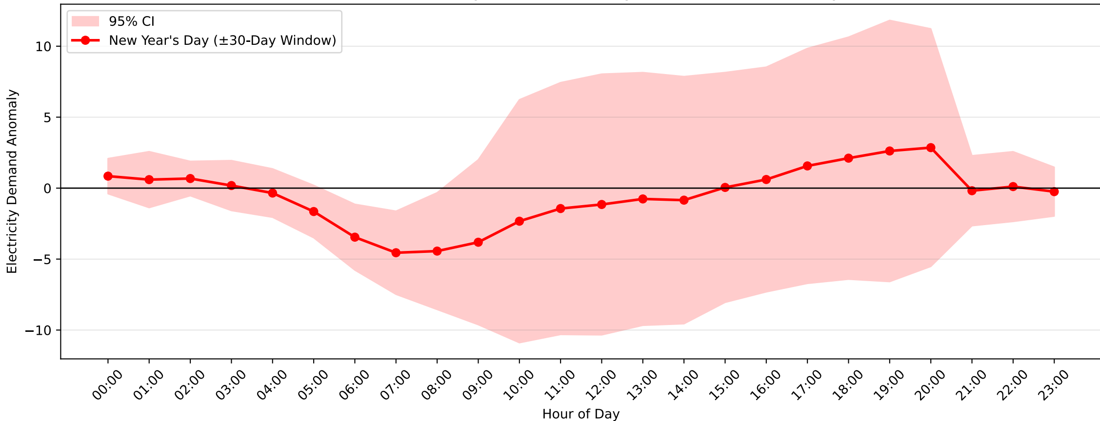
Kirrawee Demand Anomaly: New Year's Day (2005-2006, \pm 30 -Day Window)
